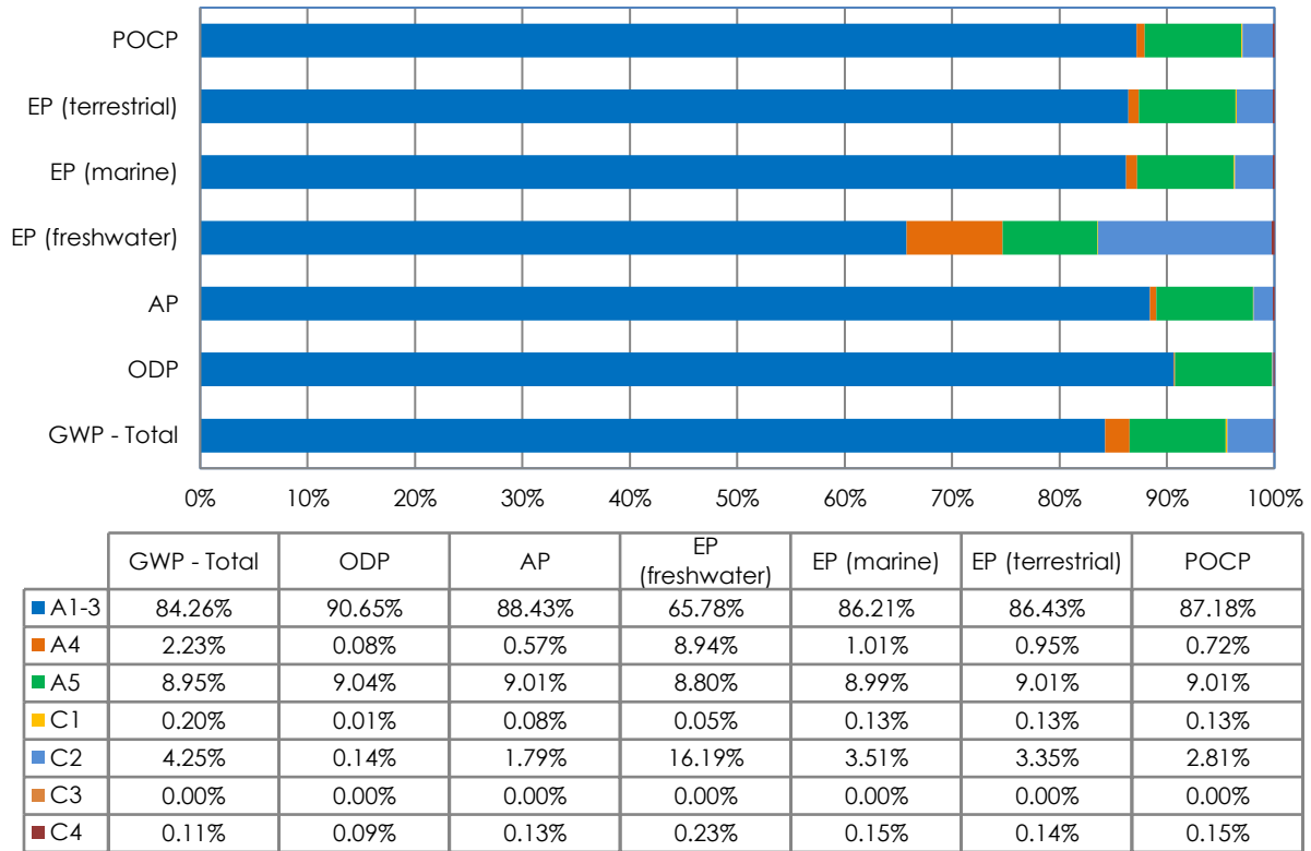
Figure 1 - shows the relative contribution of each life cycle stage to different environmental indicators for the carbon steel reinforcing bar products manufactured by the secondary (scrap based) and primary (Blast Furnace) production routes
